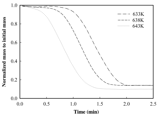
Fig. 3. Pyrolysis kinetic results of cellulose at isothermal operating temperatures of 633, 638, and 643 K.
