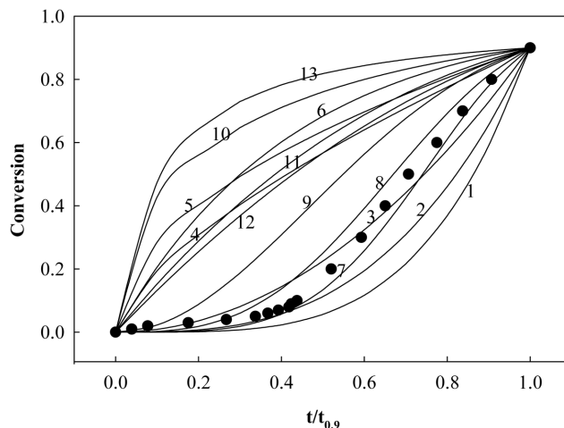
Fig. 4. Comparison of theoretical reduced time plots for reaction models defined in Table 1 with average RTP experimentally determined at three isothermal operating temperatures of 633, 638, and 643 K.
