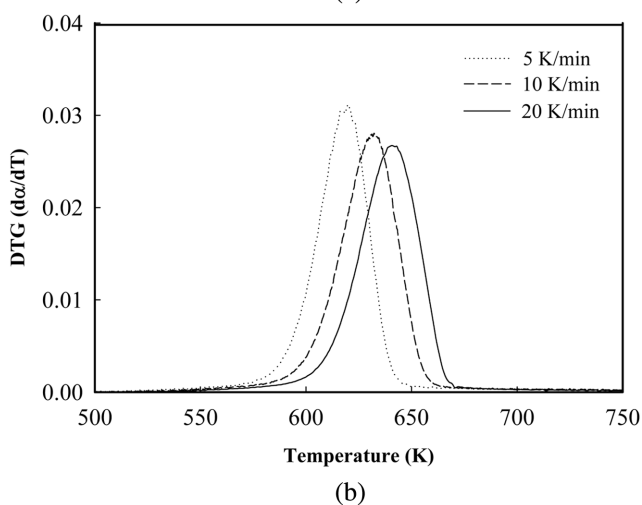
Fig. 2. TGA and DTG thermograms of cellulose under nitrogen atmosphere at the heating rates of 5, 10, and 20 K/min.
