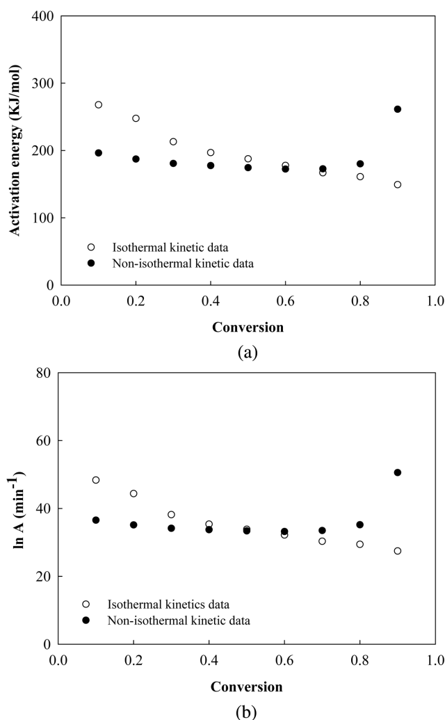
Fig. 6. Variation of activation energy and pre-exponential factor with conversion derived from two model-free methods using isothermal and non-isothermal kinetic data.
